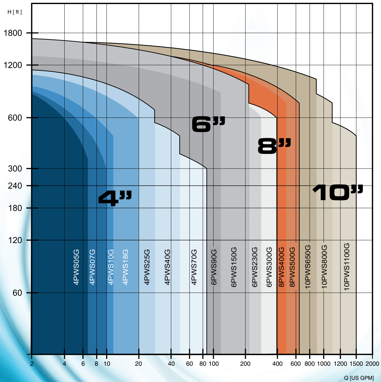
Performance range at 60 Hz
